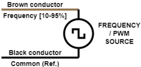
Figure 12 - Frequency input
