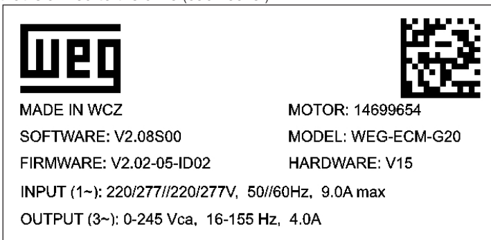
Figure 1 - Drive label
