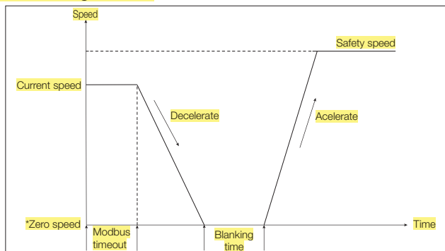
Figure 16 - Time out logic for s04 firmware version
