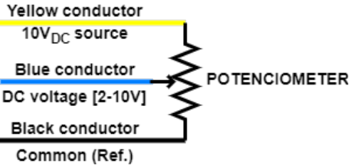
Figure 9 - DC voltage input (using built-in power supply)
