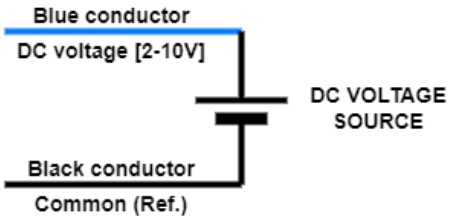
Figure 10 - DC voltage input (using external power supply)
